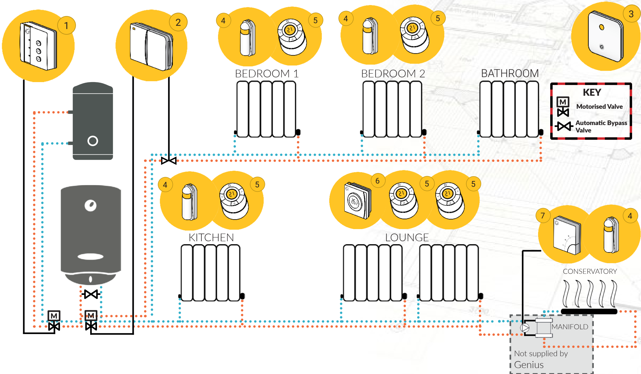
1 - Single Channel Receiver | 2 - Dual Channel Receiver | 3 - Genius Hub | 4 - Room Sensor | 5 - Radiator Valve | 6 - Room Thermostat | 7 - Electric Switch
