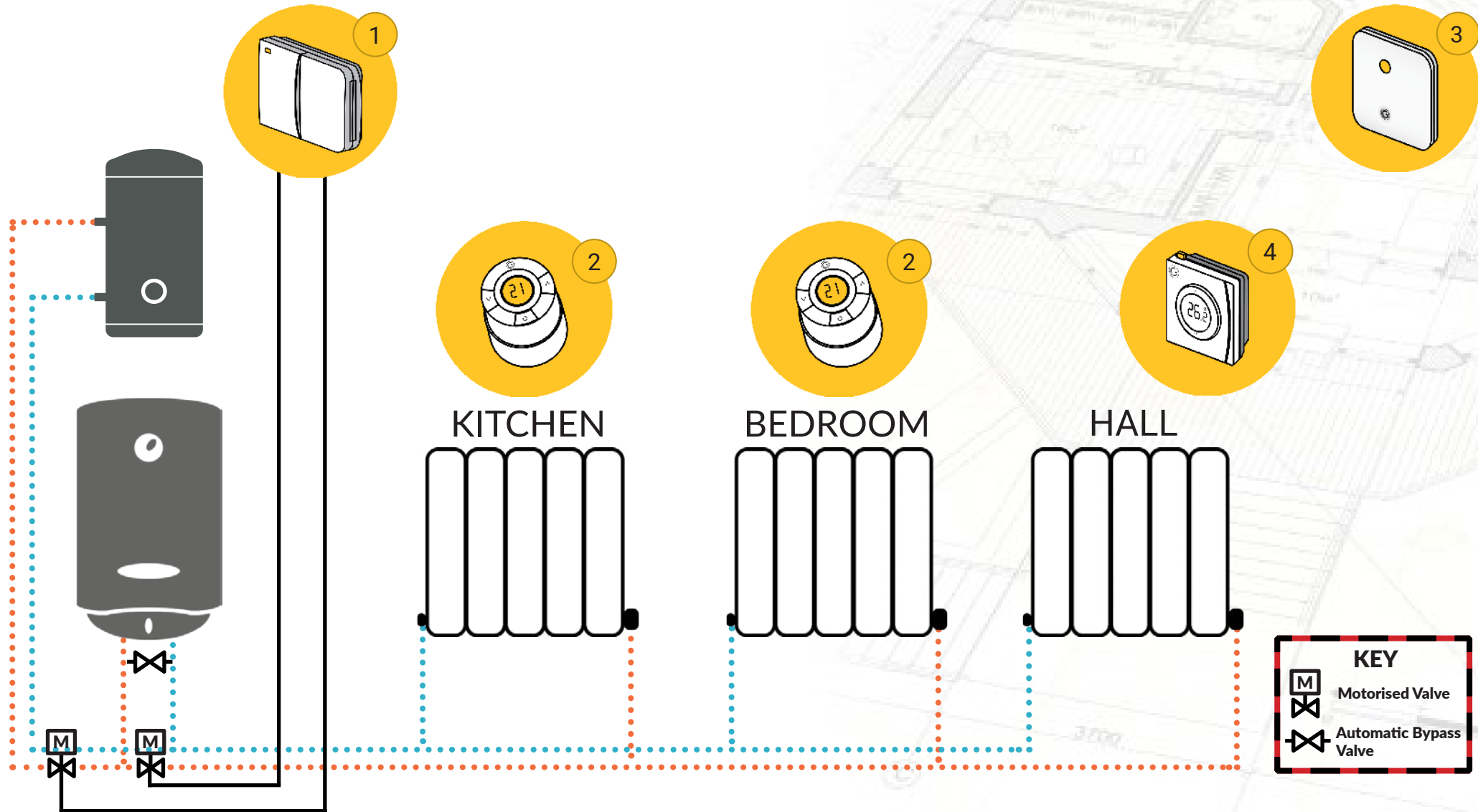
1 - Dual Channel Receiver | 2 - Radiator Valve | 3 - Genius Hub | 4 - Room Thermostat
