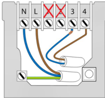
Dual Channel Receiver
