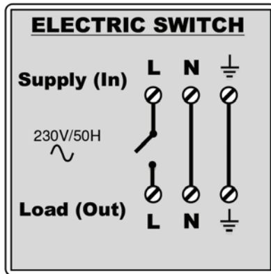
Internal Diagram
